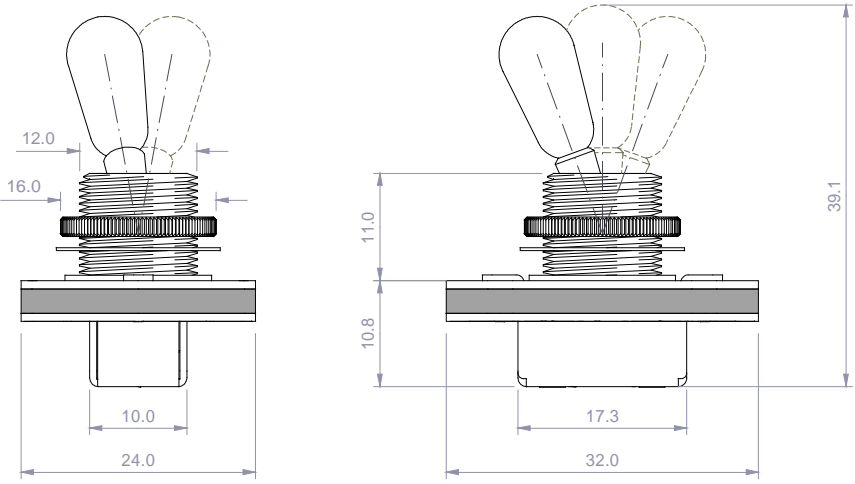
3X3-03 Schematic : Last Updated June 2013
